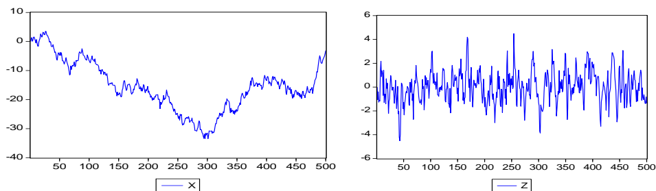
Figure 3. Properties of Times Series
