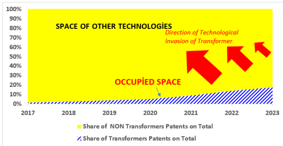
Figure 4. Patterns of morphological change in domain of large language models generated by emerging technology of transformers (Patents). Large arrows indicate the direction of technological invasion
