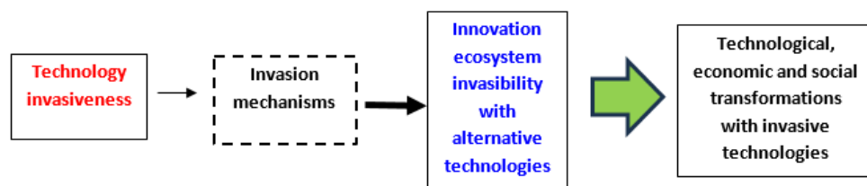
Figure 1. A Schematic diagram of invasive technologies
