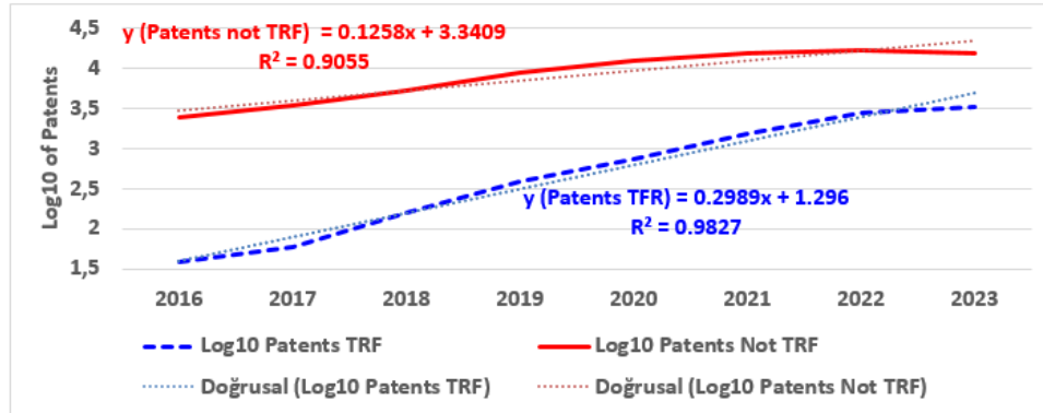
Figure 2. Estimated relationships for temporal evolution of Transformers technology compared to overall domain of large language models (Patents), 2016-2023 period. Dotted line indicates the dynamics of invasive technology; Continuous line indicates the dynamics of other alternative technologies predated.
